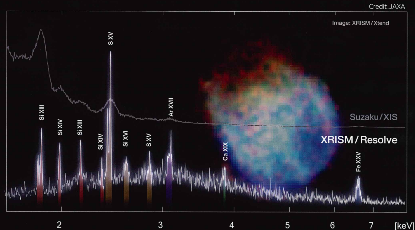
X-ray Spectrum of Supernova Remnant N132D Measured by XRISM Resolve
